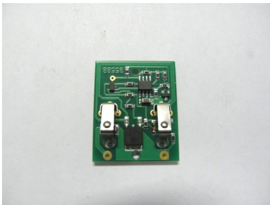
GT200850 PCB
